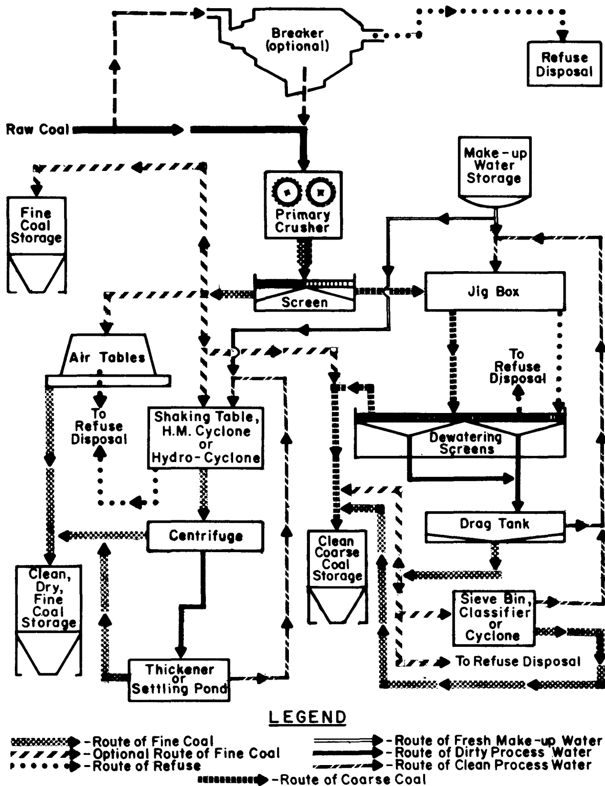
STAGE 2 - COAL PREPARATION PLANT Figure 7
