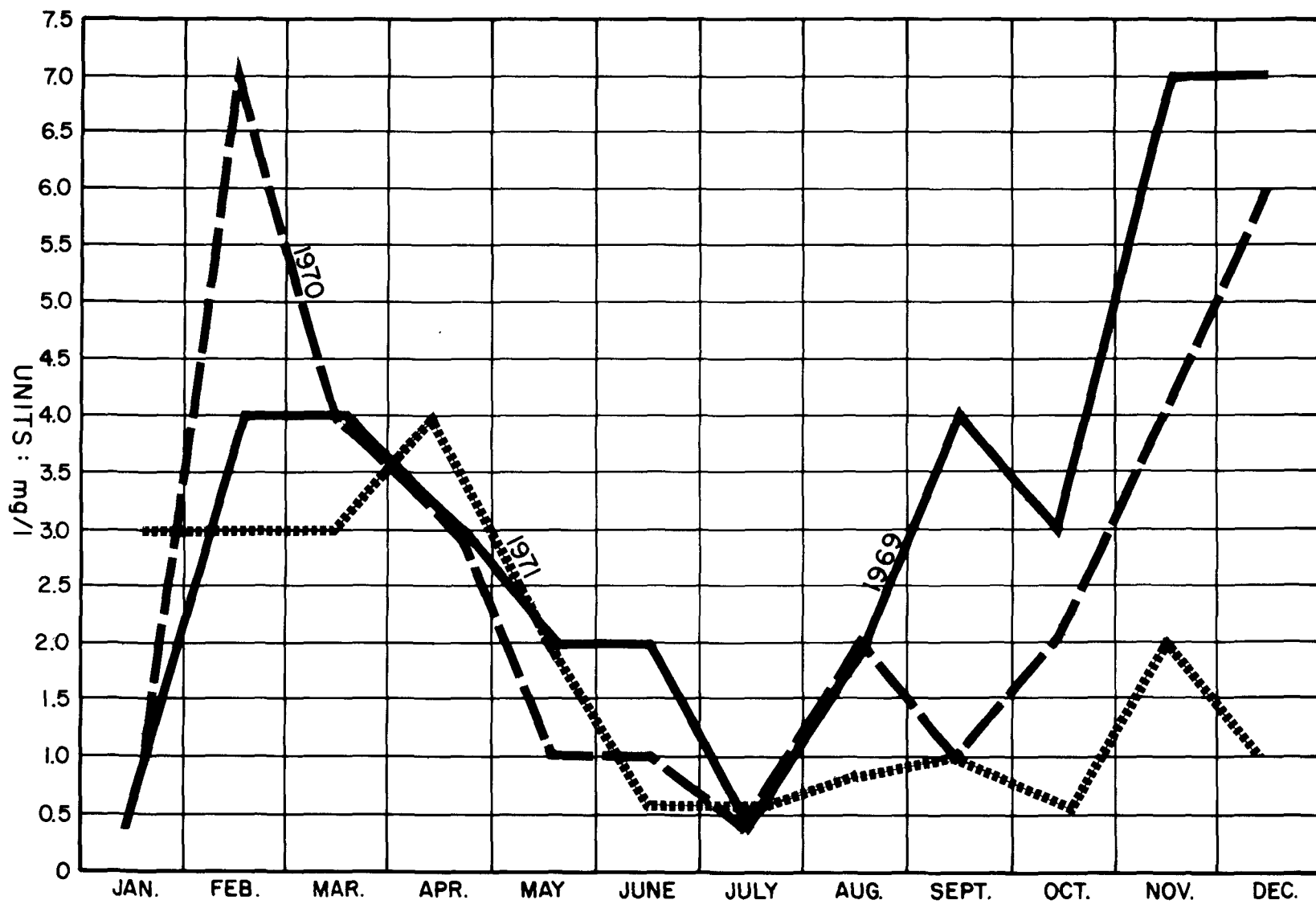
HISTORICAL DATA MONTHLY TOTAL IRON - TREATMENT PLANT A-1
